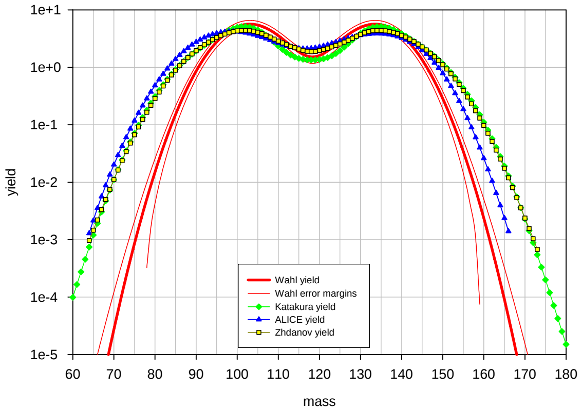
Benchmark B: ^{241}\text{Am} at 28 MeV, post neutron emission yields
